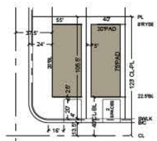
STANDARD 40'x104' LOT
