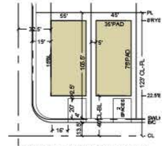
STANDARD 45'x104' LOT
