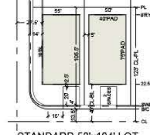
STANDARD 50'x104' LOT
