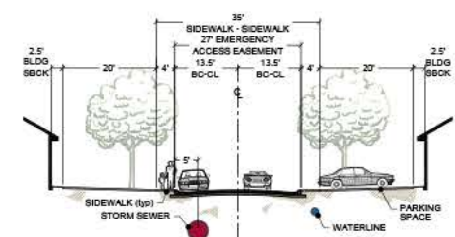
RESIDENTIAL STREET SECTION
